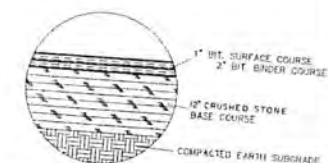
PAVING DETAIL
